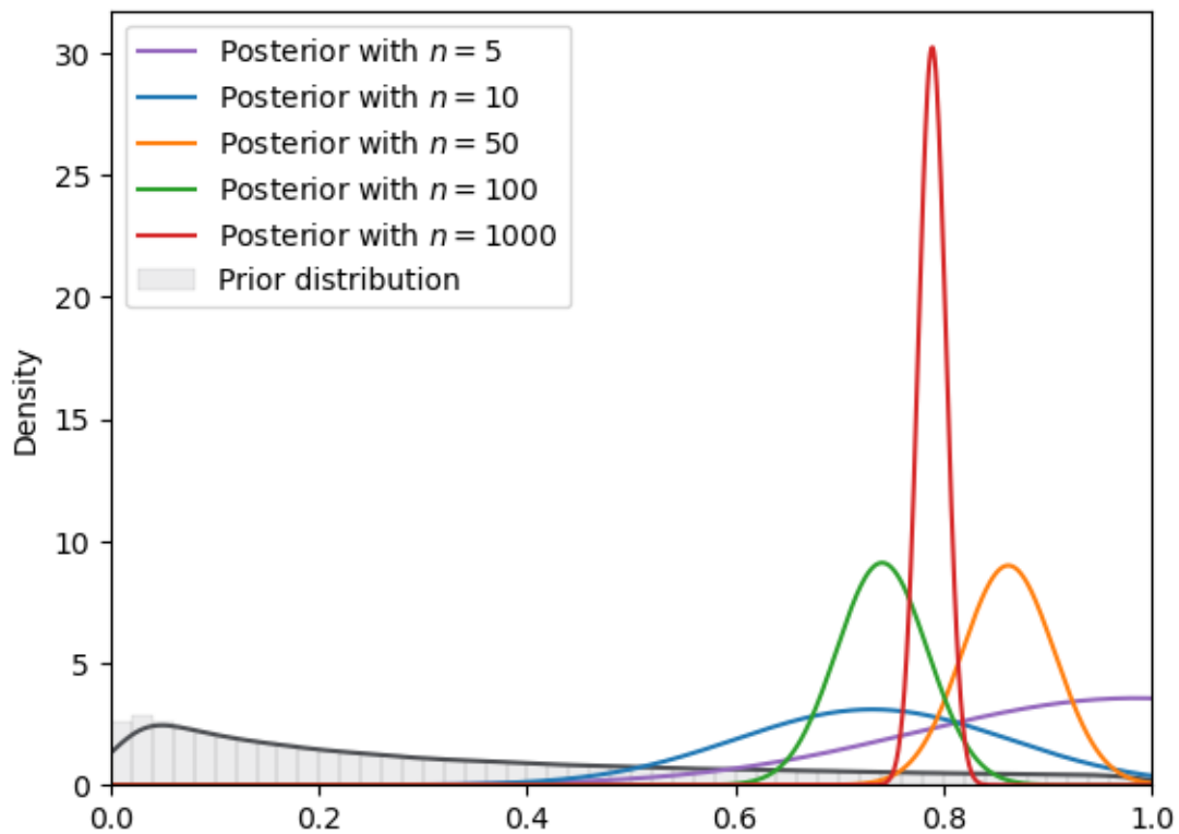
Fig. 18.14: SVI density (log normal prior, normal guide)
