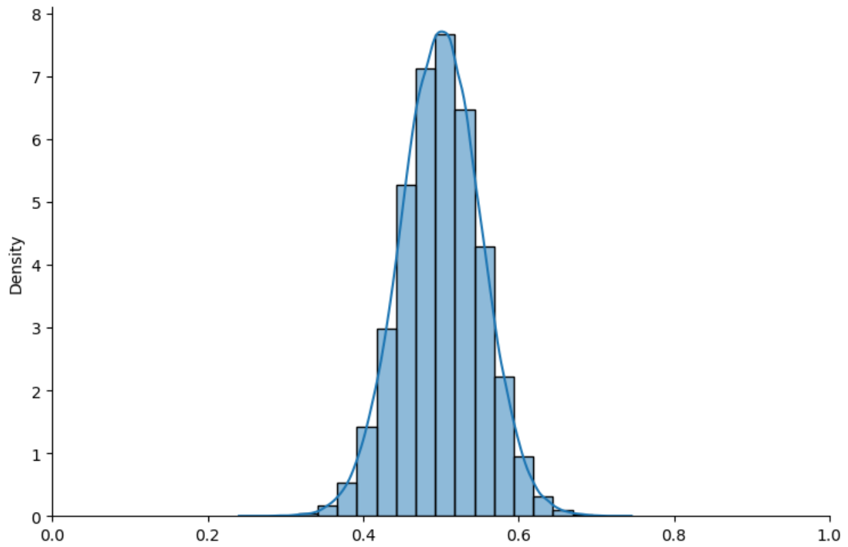
Fig. 18.3: Shifted von Mises distribution
