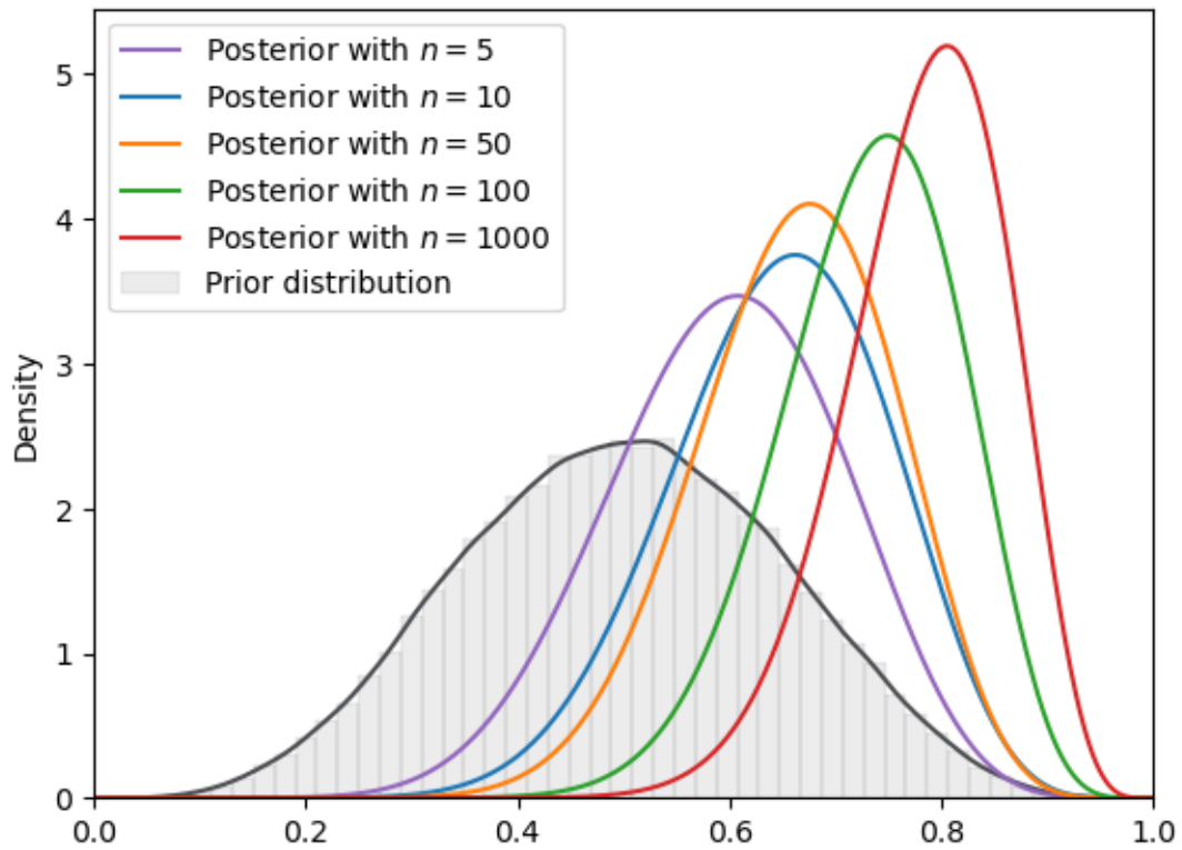
Fig. 18.7: SVI density (Beta prior, Beta guide)
