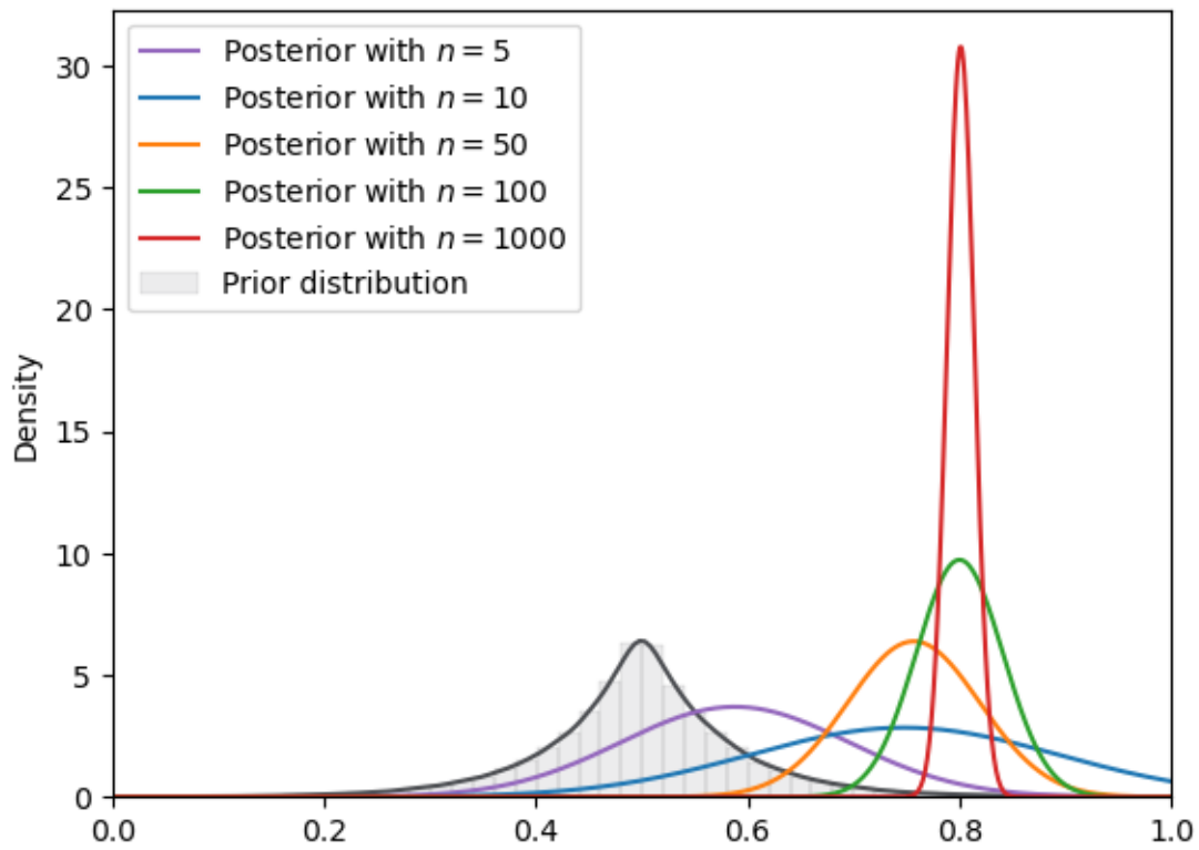
Fig. 18.15: SVI density (Laplace prior, normal guide)
