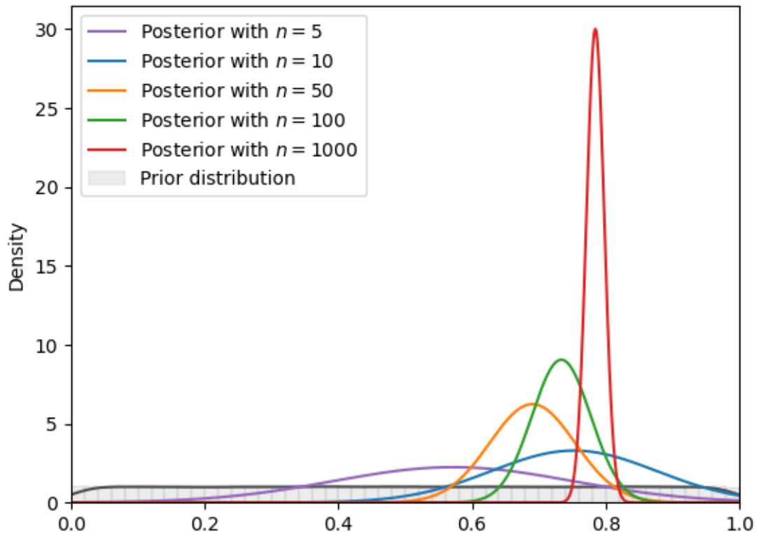
Fig. 18.13: SVI density (uniform prior, normal guide)
