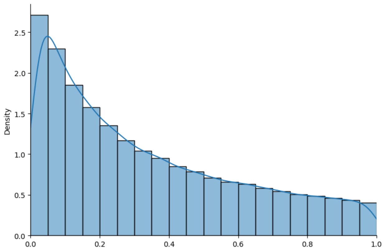
Fig. 18.1: Truncated log normal distribution
