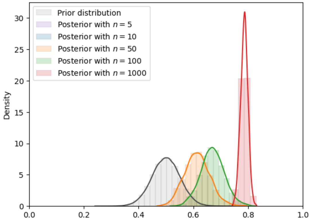
Fig. 18.11: MCMC density (von Mises prior)
