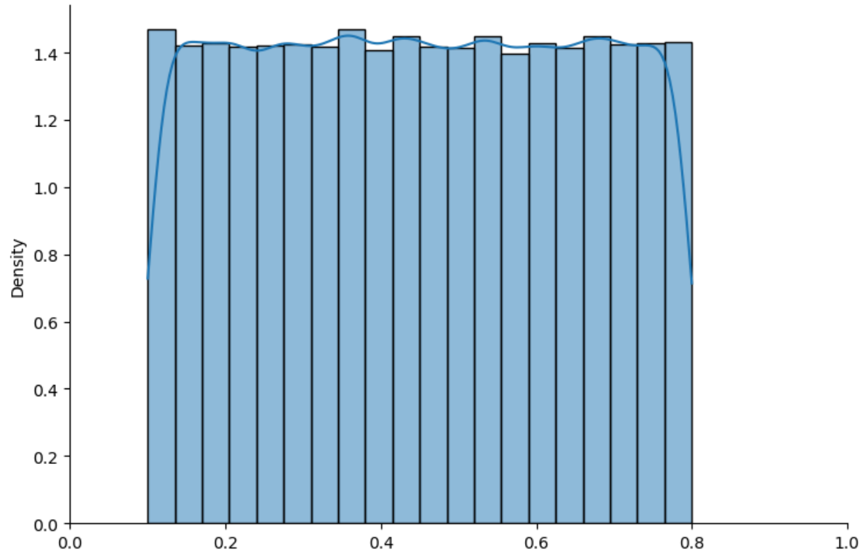
Fig. 18.2: Truncated uniform distribution
