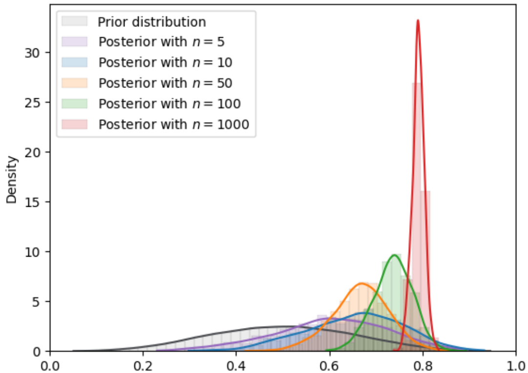
Fig. 18.6: MCMC density (Beta prior)
