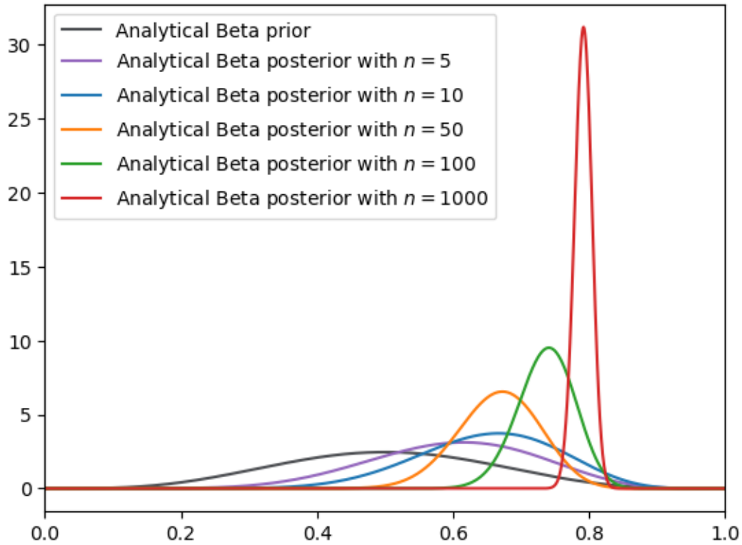
Fig. 18.5: Analytical density (Beta prior)
