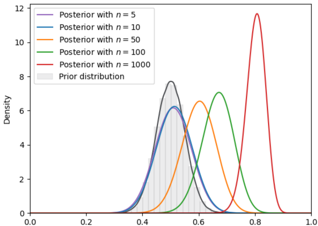
Fig. 18.18: SVI density (von Mises prior, Beta guide)
