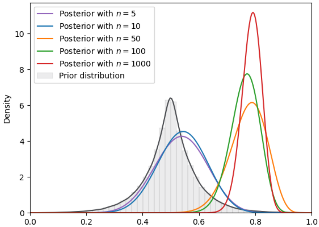
Fig. 18.19: SVI density (Laplace prior, Beta guide)
