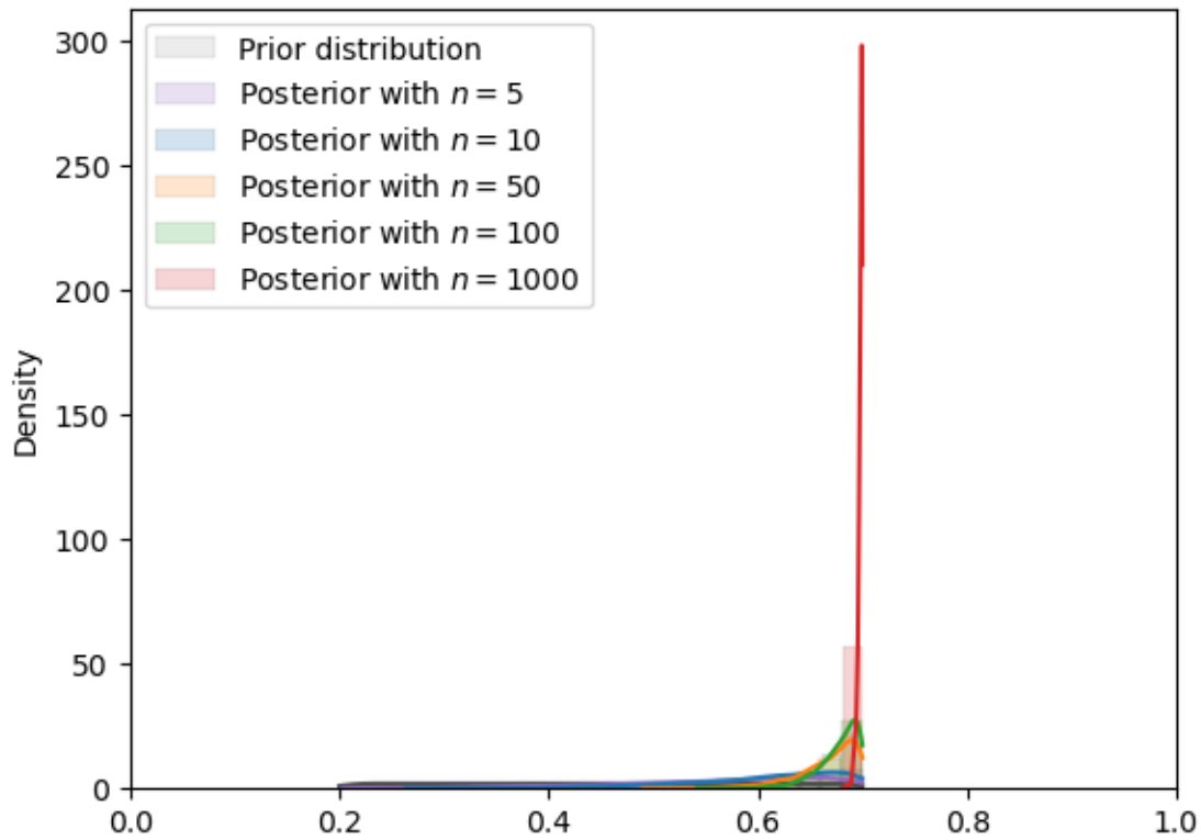
Fig. 18.9: MCMC density (uniform prior)
