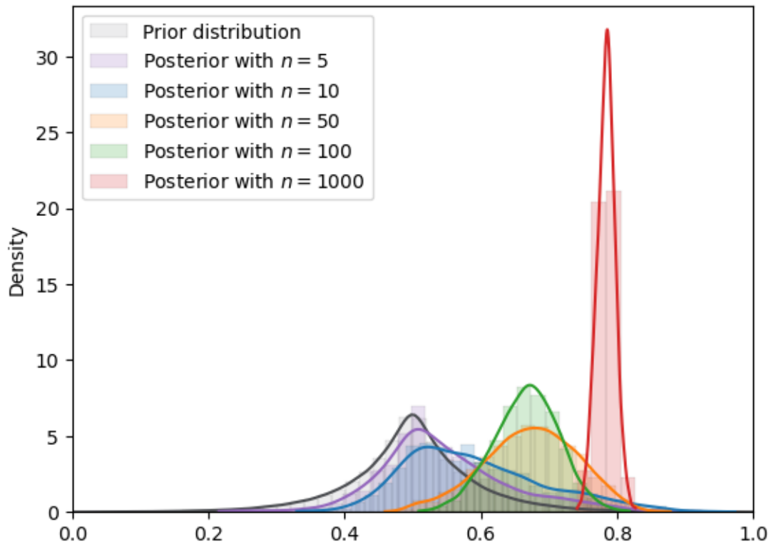
Fig. 18.12: MCMC density (Laplace prior)
