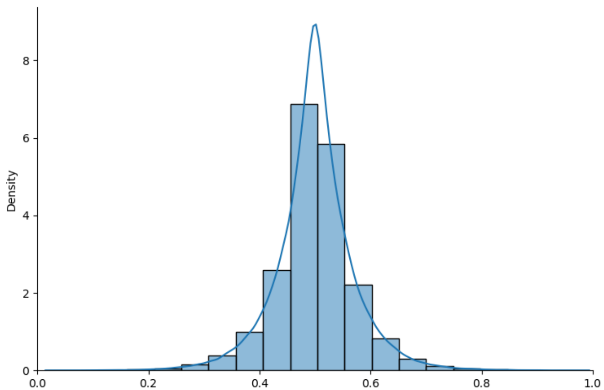
Fig. 18.4: Truncated Laplace distribution
