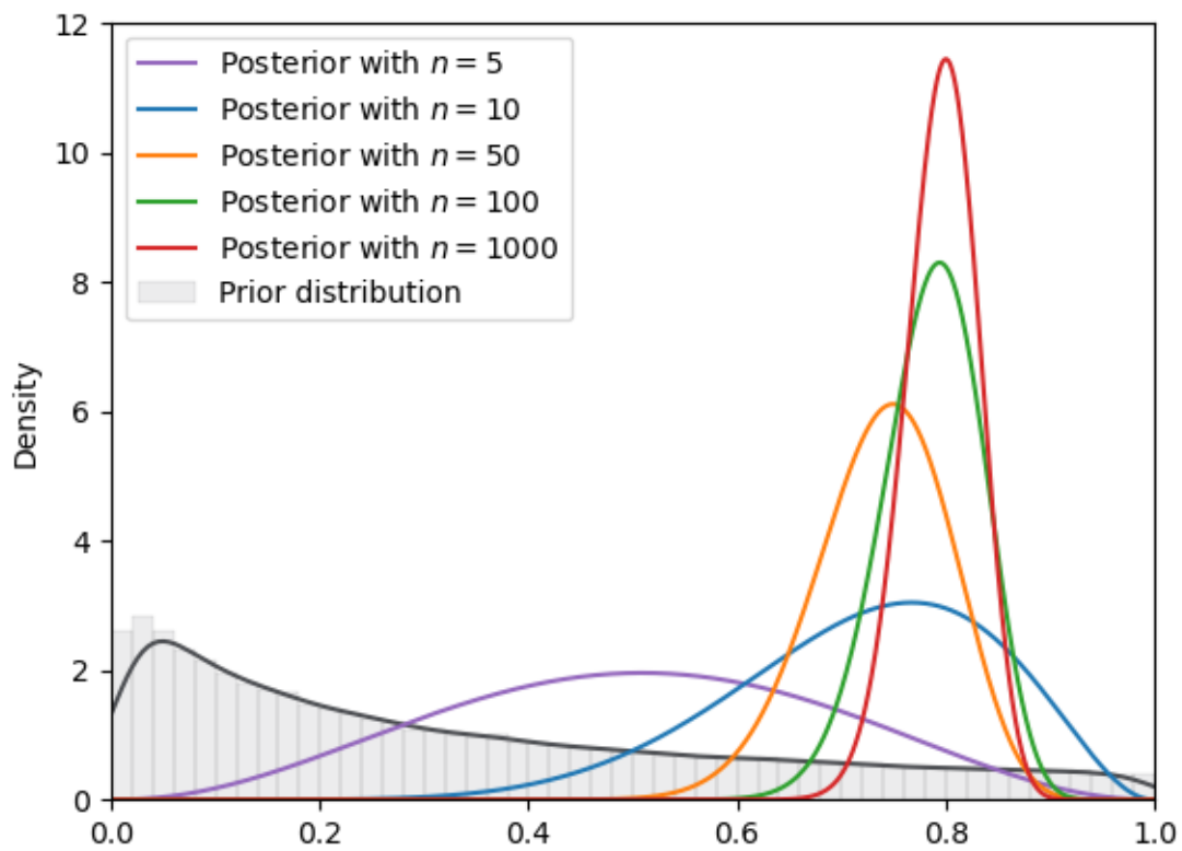
Fig. 18.17: SVI density (log normal prior, Beta guide)
