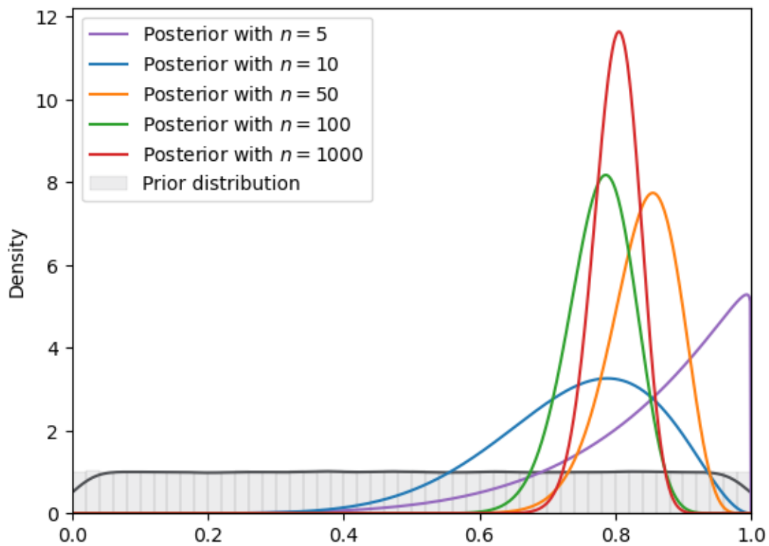
Fig. 18.16: SVI density (uniform prior, Beta guide)
