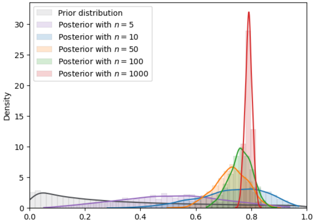
Fig. 18.10: MCMC density (log normal prior)
