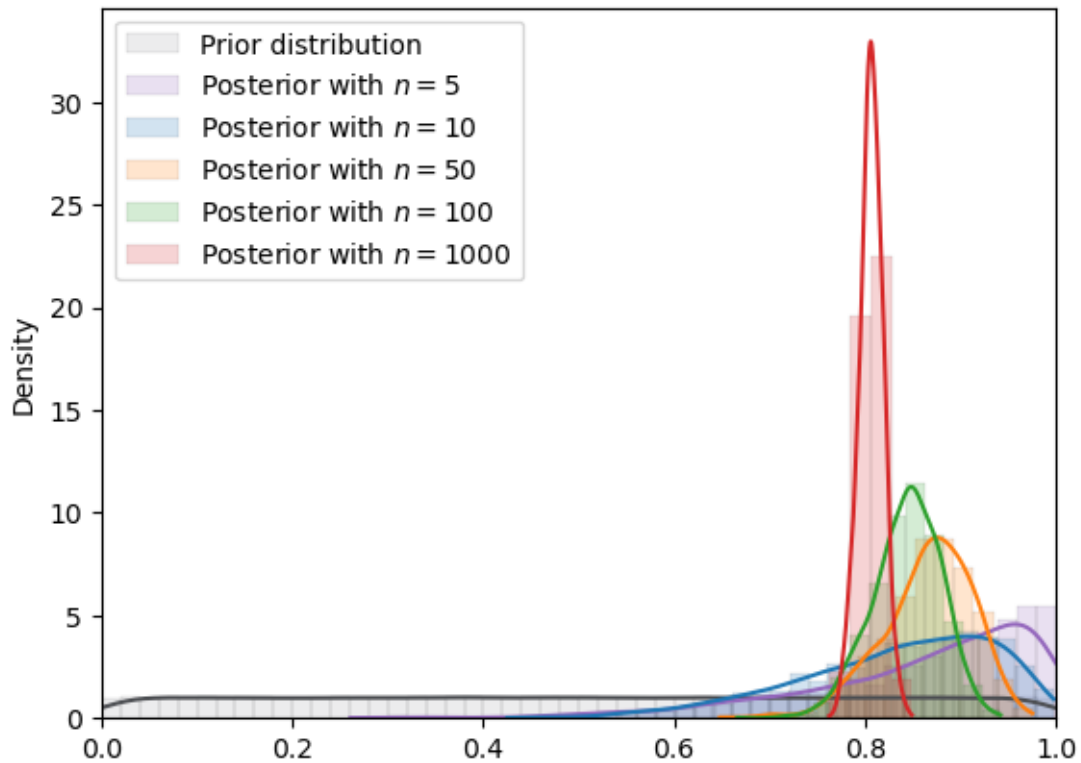
Fig. 18.8: MCMC density (uniform prior)
