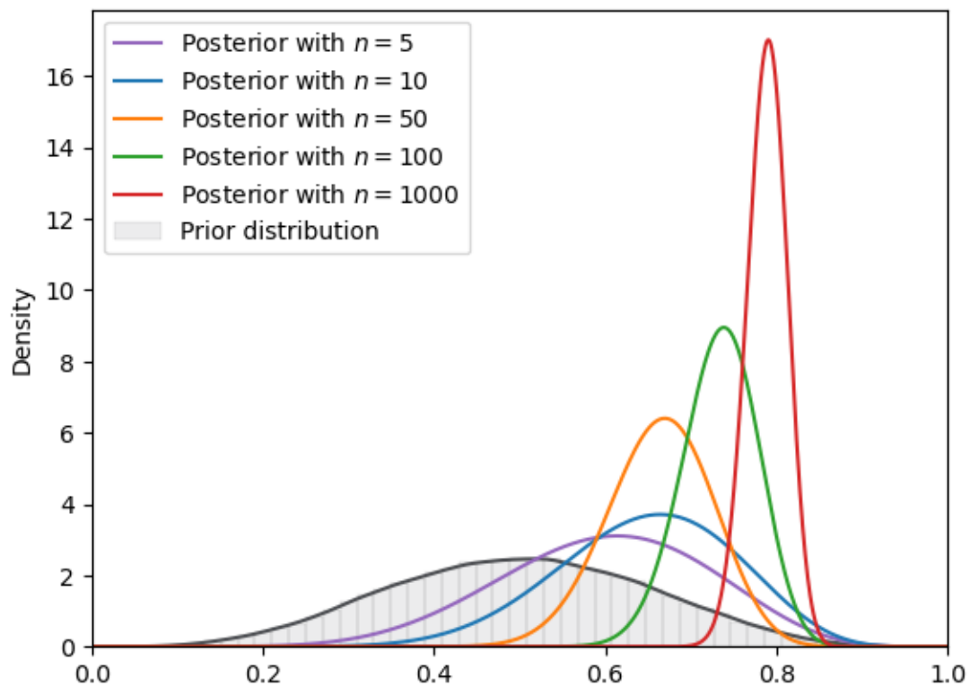
Fig. 18.7: SVI density (Beta prior, Beta guide)
